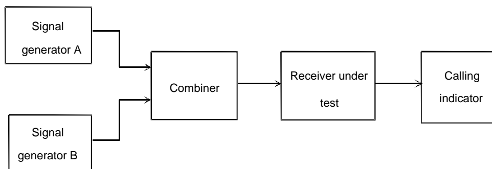
Figure 16: Measurement arrangement
