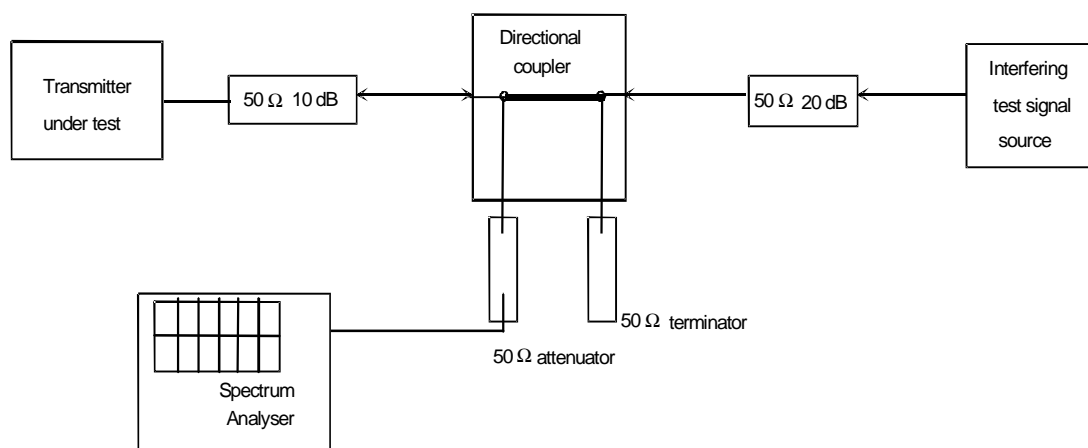
Figure 9: Measurement arrangement
