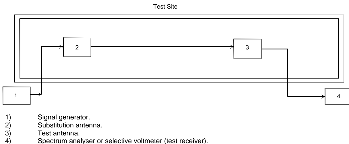
Figure 4: Measurement arrangement
