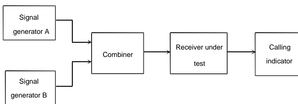
Figure 15: Measurement arrangement
